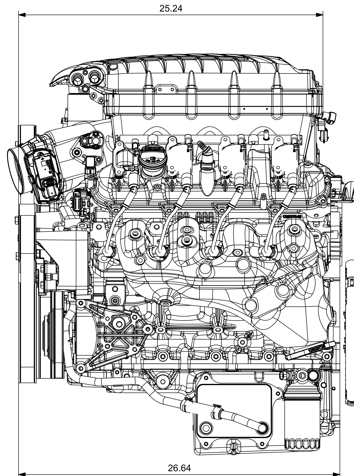
CAMARO LT OVERAL DIMENSIONS IN INCHES REGULAR LID WITH 1 INCH SPACER
