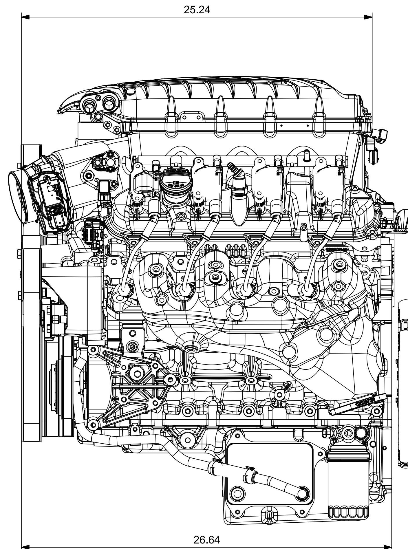
CAMARO LT OVERAL DIMENSIONS IN INCHES REGULAR LID
