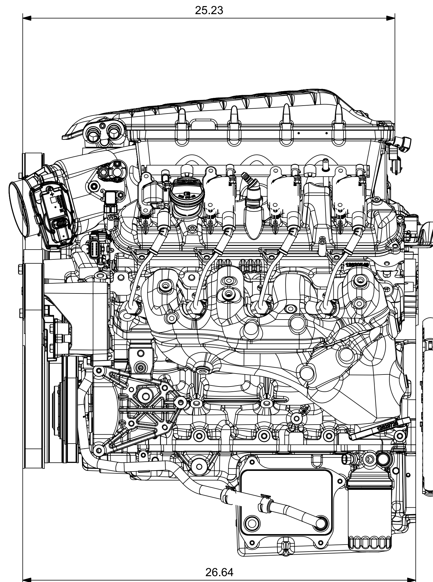
CAMARO LT OVERAL DIMENSIONS IN INCHES ULTRA-LOW LID
