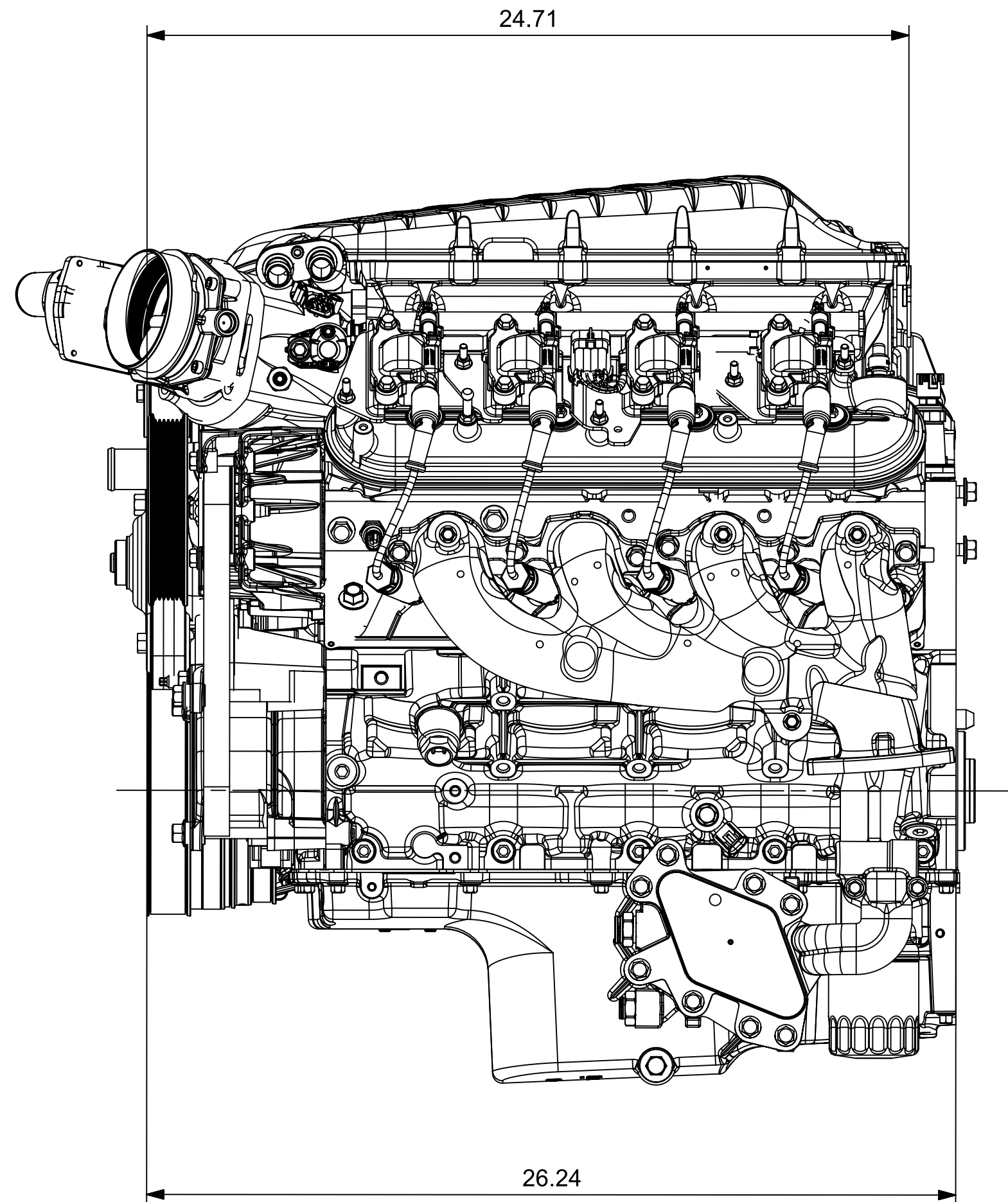
CAMARO LS OVERAL DIMENSIONS IN INCHES ULTRA-LOW LID
