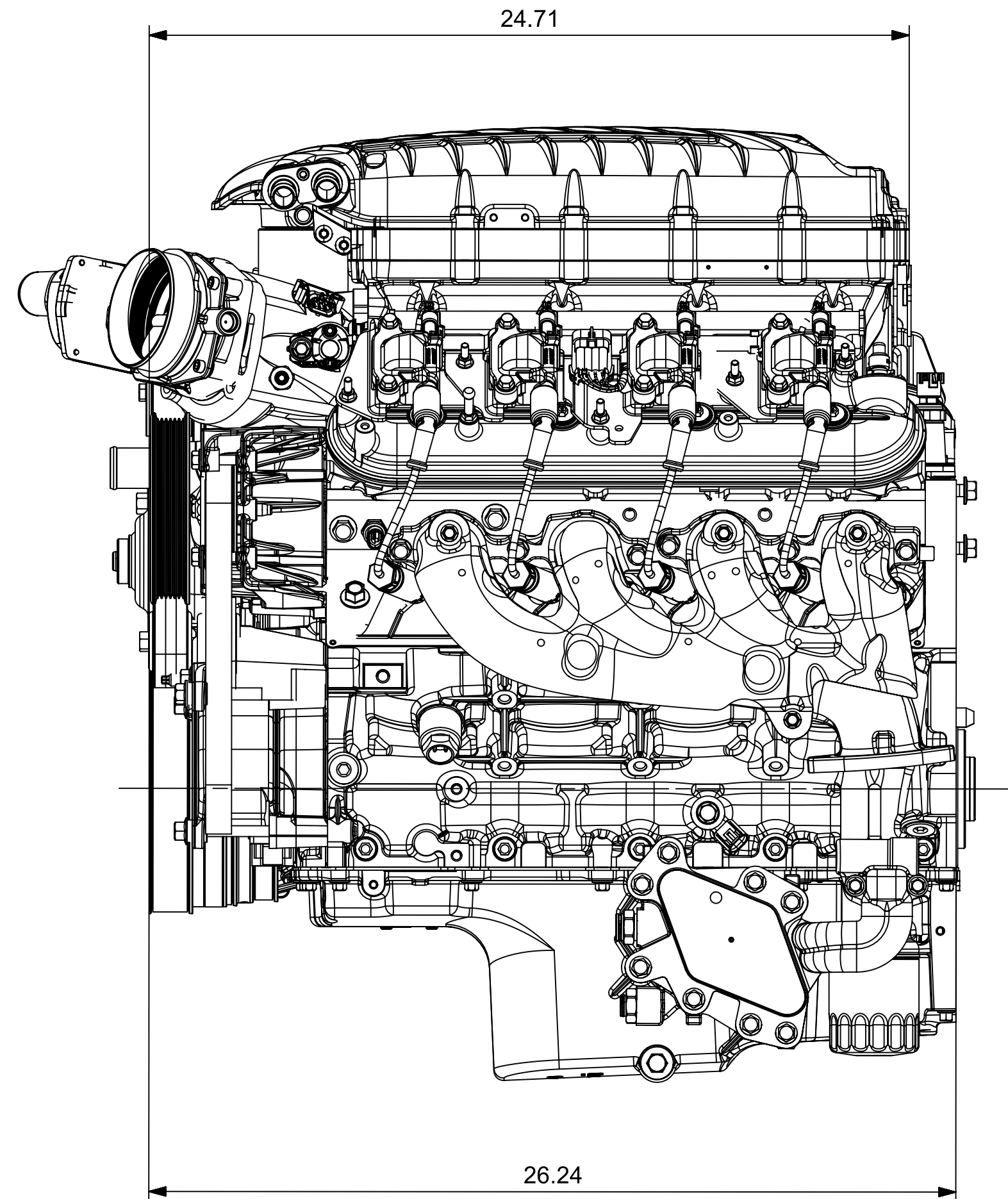
CAMARO LS OVERAL DIMENSIONS IN INCHES REGULAR LID WITH 1 INCH SPACER
