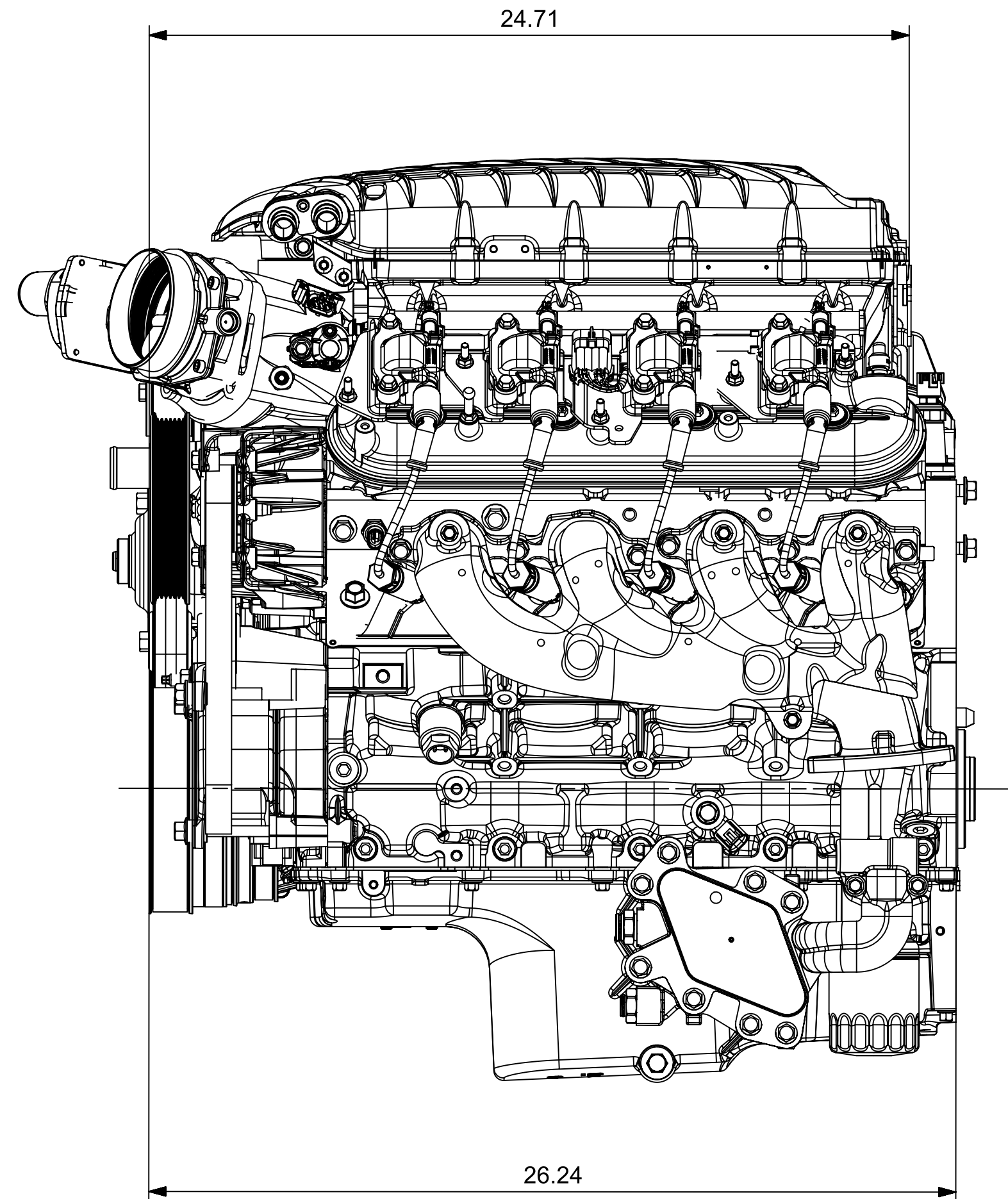
CAMARO LS OVERAL DIMENSIONS IN INCHES REGULAR LID
